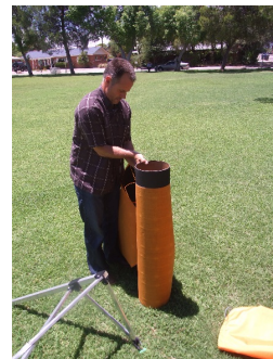
Wrap solar panel around the packaging tube
